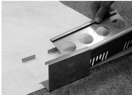
Ballasted retainer and connector for aluminum angle profile DP 80-A
